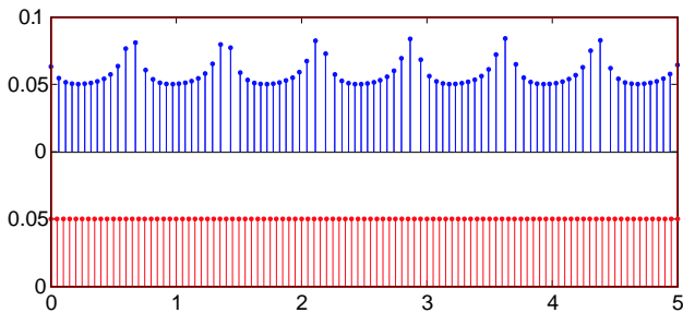
Figure 3. Activation times for the control-driven and periodic controller
